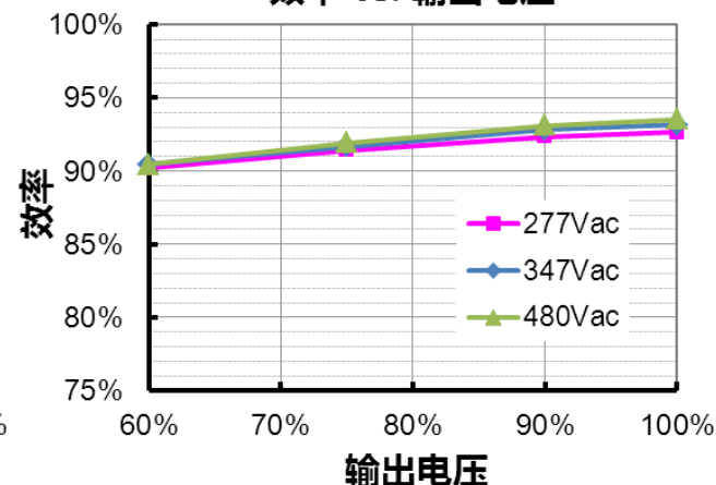
ESD-480S280DT (Io=2800mA) 效率 vs. 输出电压
