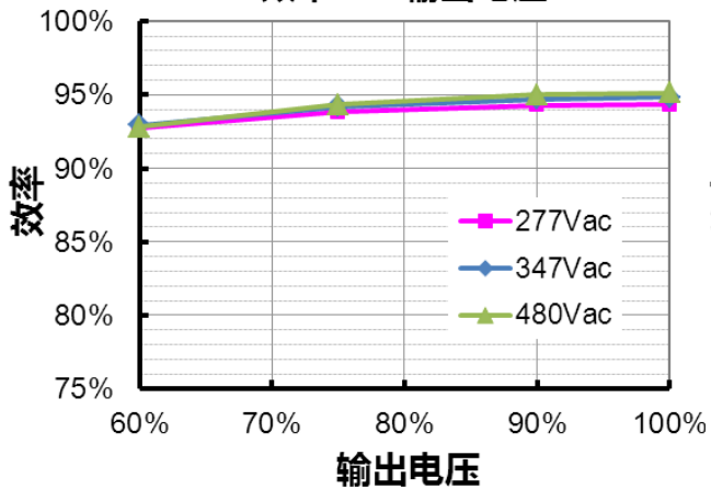
ESD-480S420DT (Io=3150mA) 效率 vs. 输出电压
