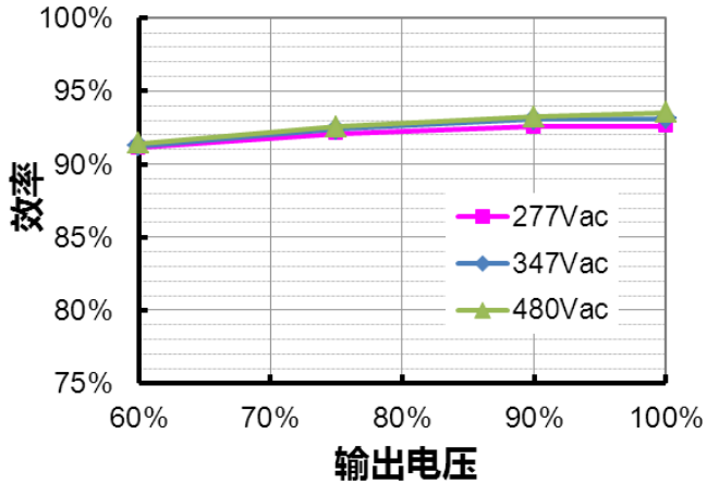
ESD-480S560DT (Io=4350mA) 效率 vs. 输出电压
