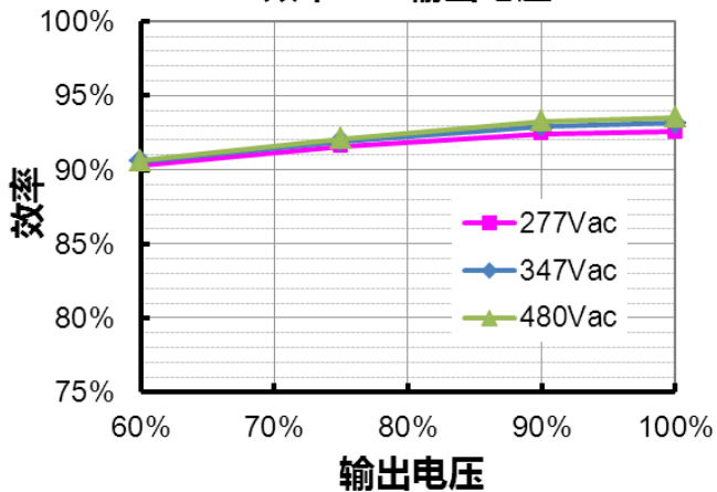
ESD-480S10ADT (Io=7500mA) 效率 vs. 输出电压
