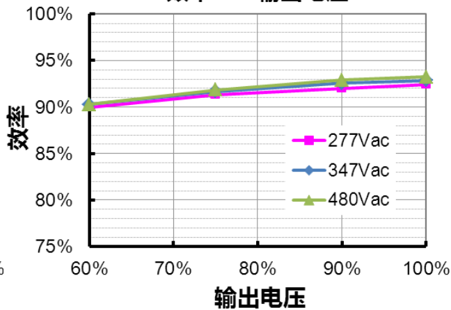
ESD-480S420DT (Io=4200mA) 效率 vs. 输出电压
