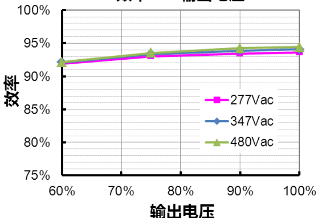
ESD-480S280DT (Io=2100mA) 效率 vs. 输出电压
