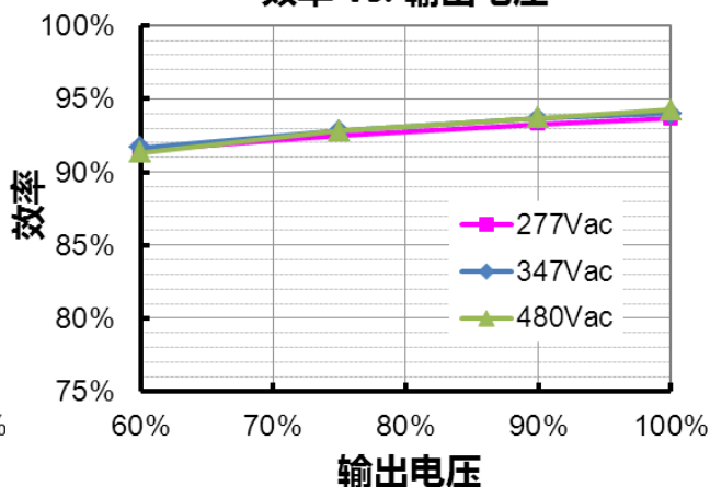
ESD-480S140DT (Io=1400mA) 效率 vs. 输出电压
