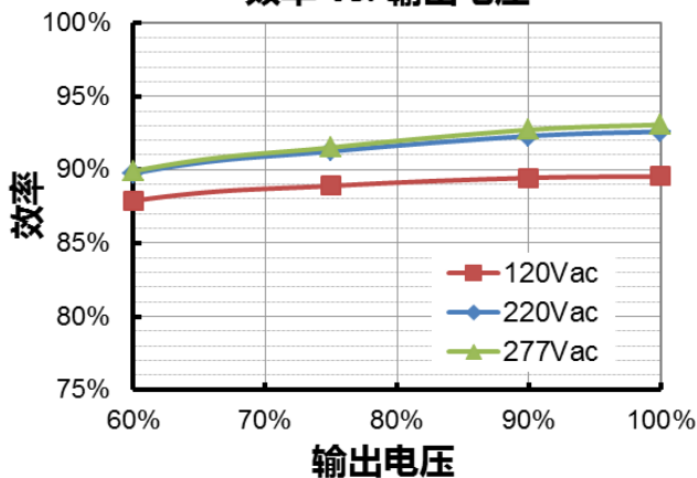
EUK-240S420DT(TT)( I_o=2800mA ) 效率 vs. 输出电压
