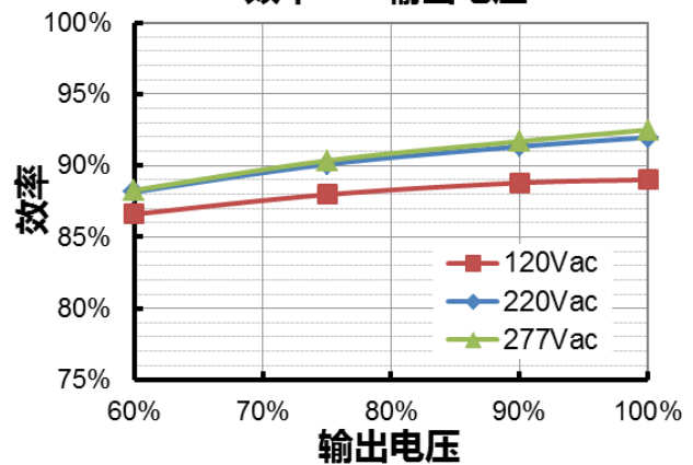
EUK-240S210DT(TT)( I_o=2100mA ) 效率 vs. 输出电压
