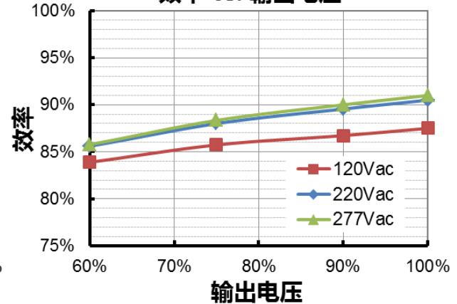
EUK-240S420DT(TT)( I_o=4200mA ) 效率 vs. 输出电压
