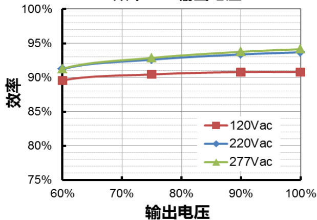
EUK-240S210DT(TT)( I_o=1400mA ) 效率 vs. 输出电压
