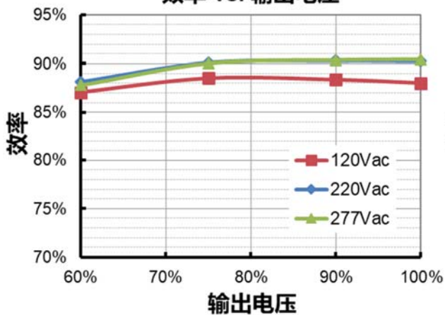
EAM-100S280SB( I_o=1750mA ) 效率 vs. 输出电压
