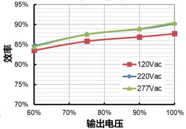
EAM-100S280SB( I_o=2800mA ) 效率 vs. 输出电压
